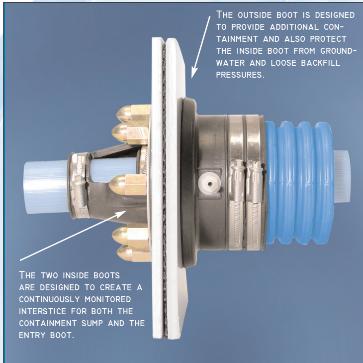
The outside boot seals to the primary, secondary or chase pipe
