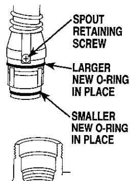
FIG. 1 NEW SPOUT ASSEMBLY
