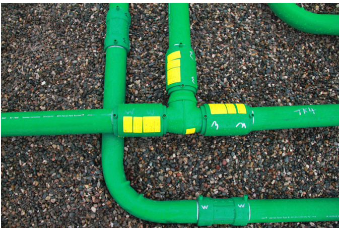
KPS' compact fittings allow for easy, fast welds
