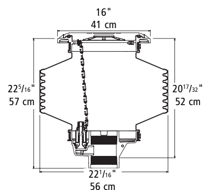
OPW 1-2115, 15-Gallon
