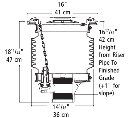
OPW 1-2100, 5-Gallon
