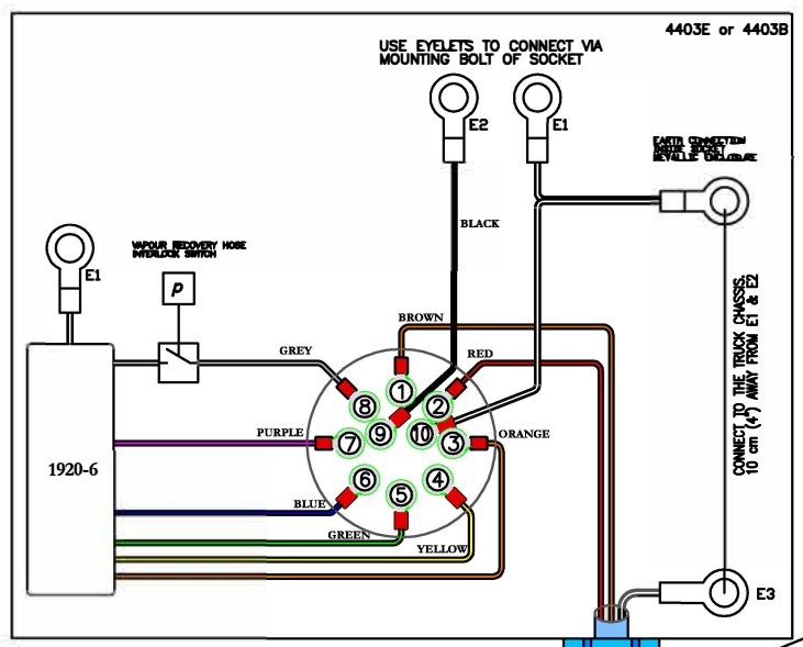
SOCKET VIEW FROM WIRE CONNECTION SIDE
