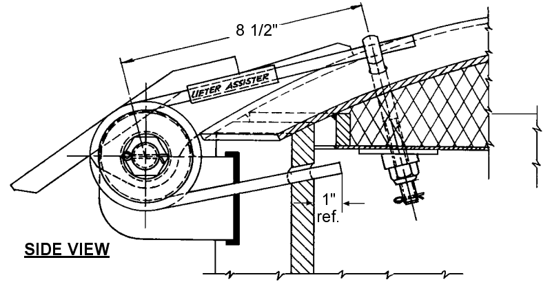
TYPICAL INSULATED COVER ARRANGEMENT
