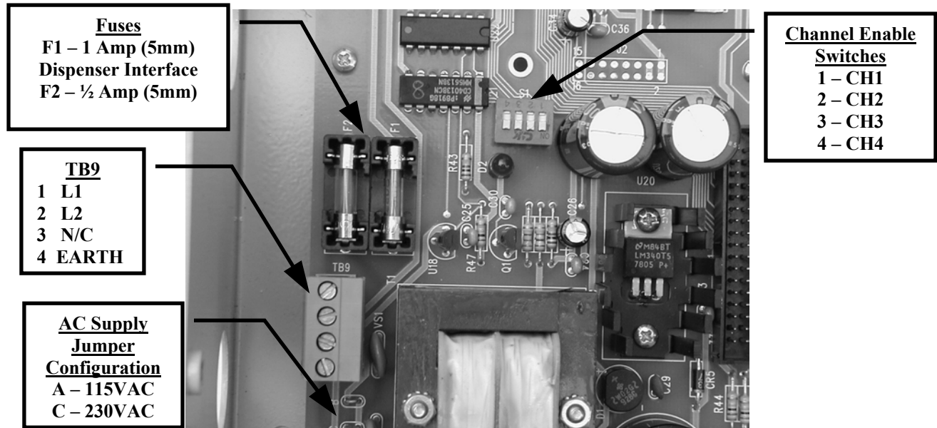
Figure 13 - AC Supply Power Connections
